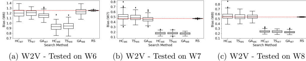
Figure 1: RQ1: Boxplots of gender bias values (the lower the better) achieved by the single-objective search algorithms (HC, TS, GA) and RS over 100 runs. The dashed (red) line indicates the gender bias value of the original pre-trained model baseline.
