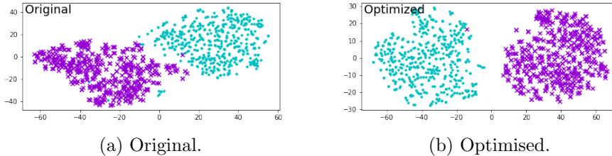
Figure 2: RQ1: Visualization of bias mitigation effectiveness with tSNE. (a) shows the most male-biased and female-biased vectors of the original, pre-trained W2V model; (b) shows vectors after optimisation obtained using Tabu Search with WEAT 6 as a training set.
