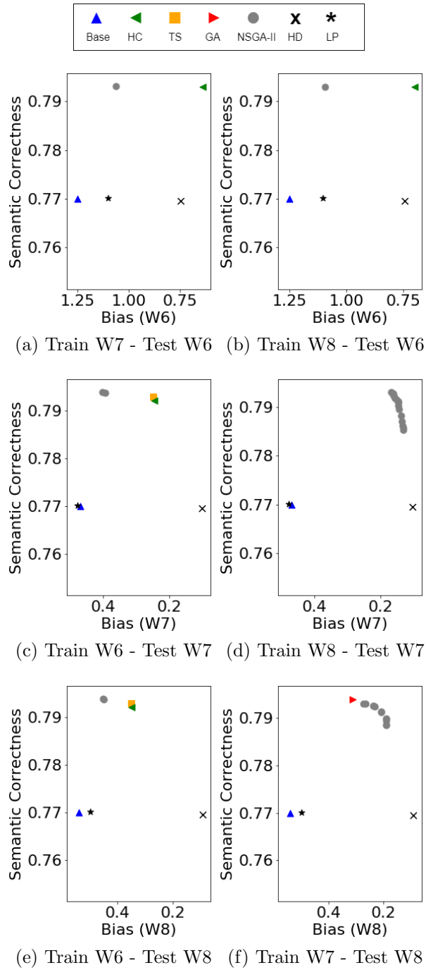
Figure 3: RQ3: Bias and semantic correctness achieved by the Base original word embedding model, NSGA-II (circle) and WSM (filled markers), and the state-of-the-art HD and LP.
