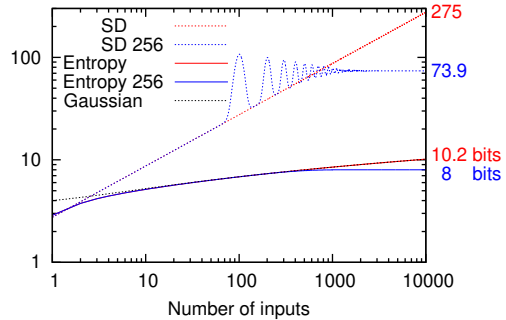
Figure 10: Standard deviation and entropy of adding 0-9. Figure 8 upper red convergence to Gaussian, entropy \log_2(\sigma) + 2.0471 . Figure 9 lower blue, forced into 8 bit arithmetic sum converges to uniform 0-255, entropy 8 bits.
