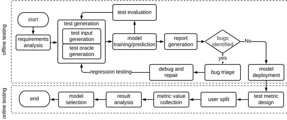
Figure 5: Idealised Workflow of ML testing
